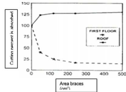
Fig: 17. Area braces absorbed by the frame effect on percent cut
