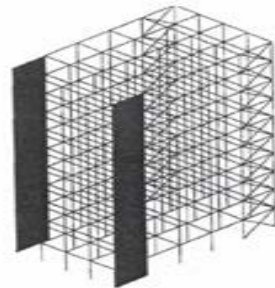
Fig. 3. The second stage analysis of frame and shear walls(fw1)
