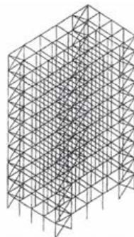
Fig. 5. The third stage frame analysis and bracing
