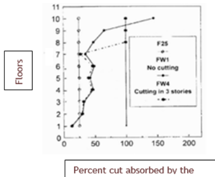
Fig. 9 . The effect of shear walls cut at the top on cutting absorbed by the frame
