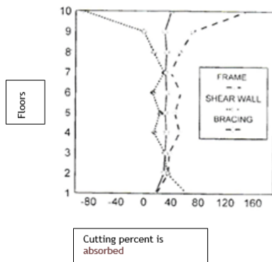
Fig:13. Interaction frame, shear wall and bracing (structures fwb1)
