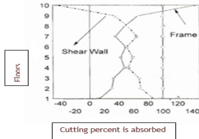
Fig. 8. linteraction frame - double shear (structural fw1)
