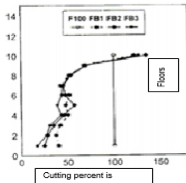
Fig: 16-area braces absorbed by the frame effect on percent cut
