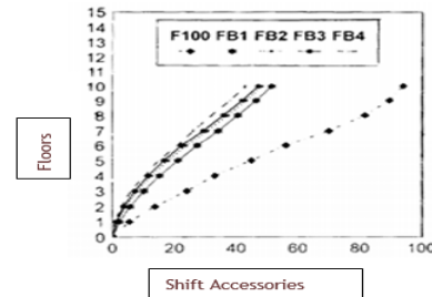
Fig:14. Area bracing effect on the lateral displacement (stage iv)
