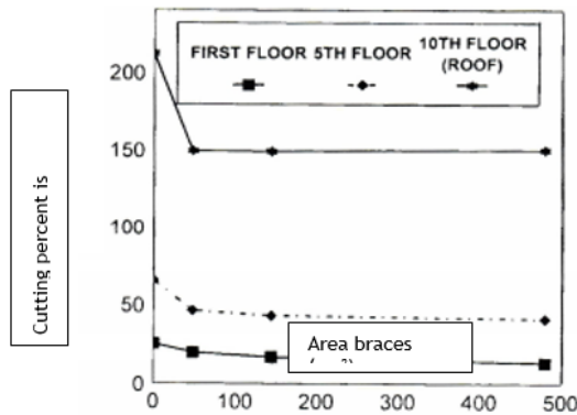
Fig:12. The impact on the absorption area braces for earthquake by frame (the third stage of analysis)
