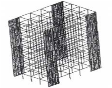
Fig. 3. The second stage analysis of frame and shear walls(fw1)
