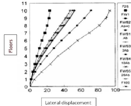
Fig.10. Area bracing effect on the lateral displacement (stage iii)
