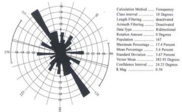
Figure6: Rose diagram related on Surmehmountain
