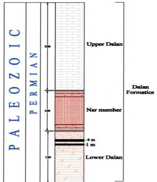
Figure 4 :Geological formation of the Surmeh mountain.
