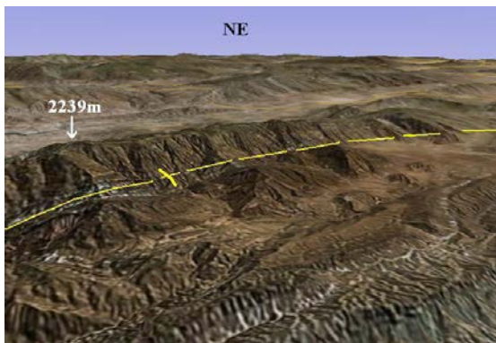
Figure2: View Northeast across Surmeh anticline in the Surmeh mountain, SW, Shiraz, Iran. showing the highest elevation. The scale is indicated by the length of anticline
