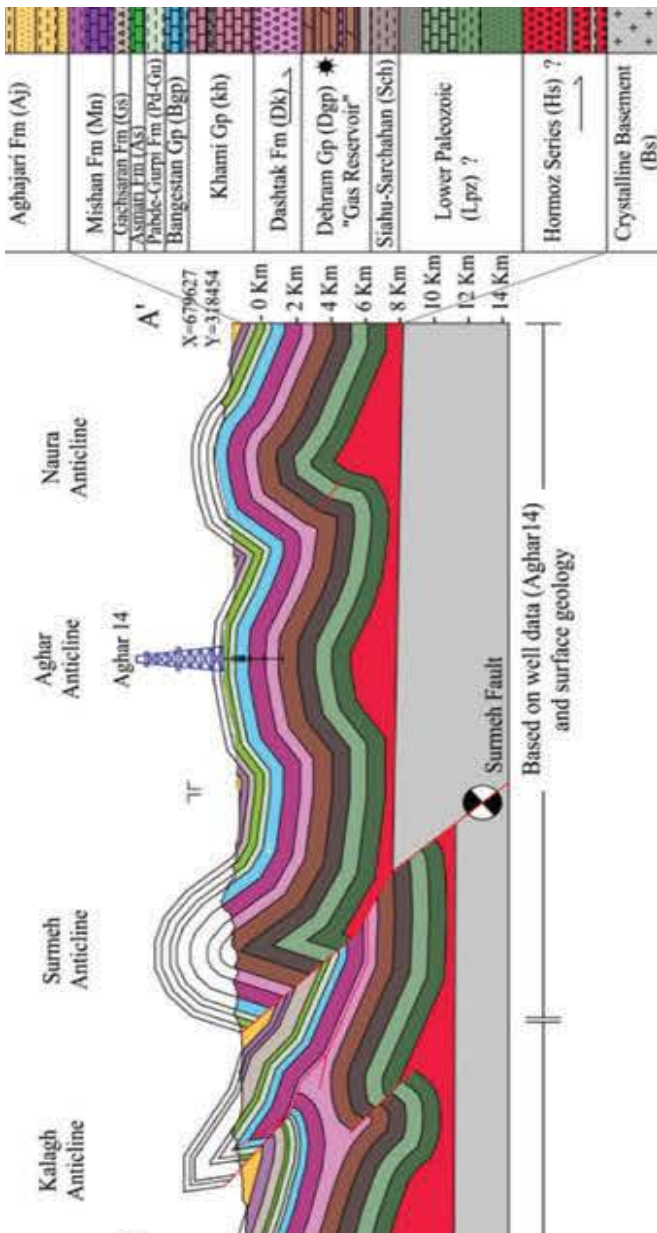
Figure 5: Geological formation of the Surmeh anticline
