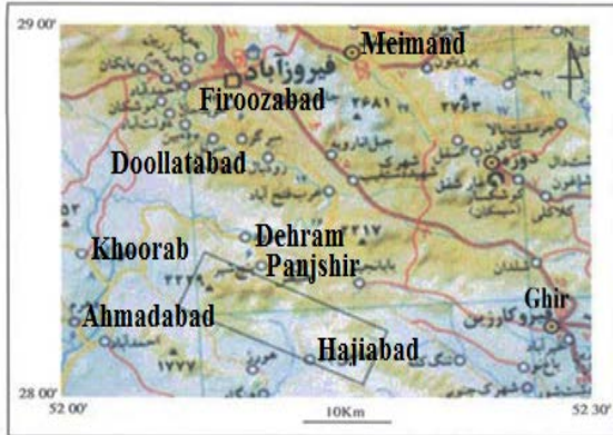
Figure 1: Location of the Surmeh, and the area studied in the present paper paper
