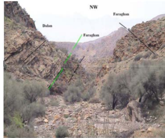
Figure 3: Geological formation of Surmeh anticline in Surmeh anticline, SW, Shiraz, Iran, showing geological formation. The scale is indicated by the vegetation. Northwest view of the Surmehmountain. The scale is indicated by the vegetation
