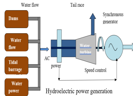
Figure 6. Hydroelectric power stations: These convert hydro energy to electrical energy.
